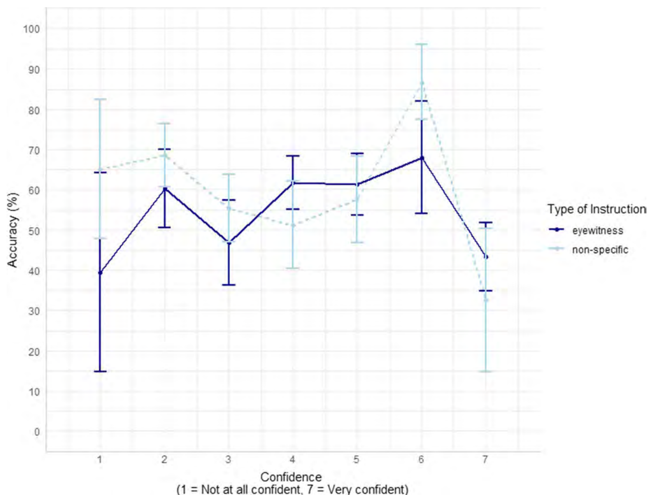
Fig. 3: 7-bin CAC
