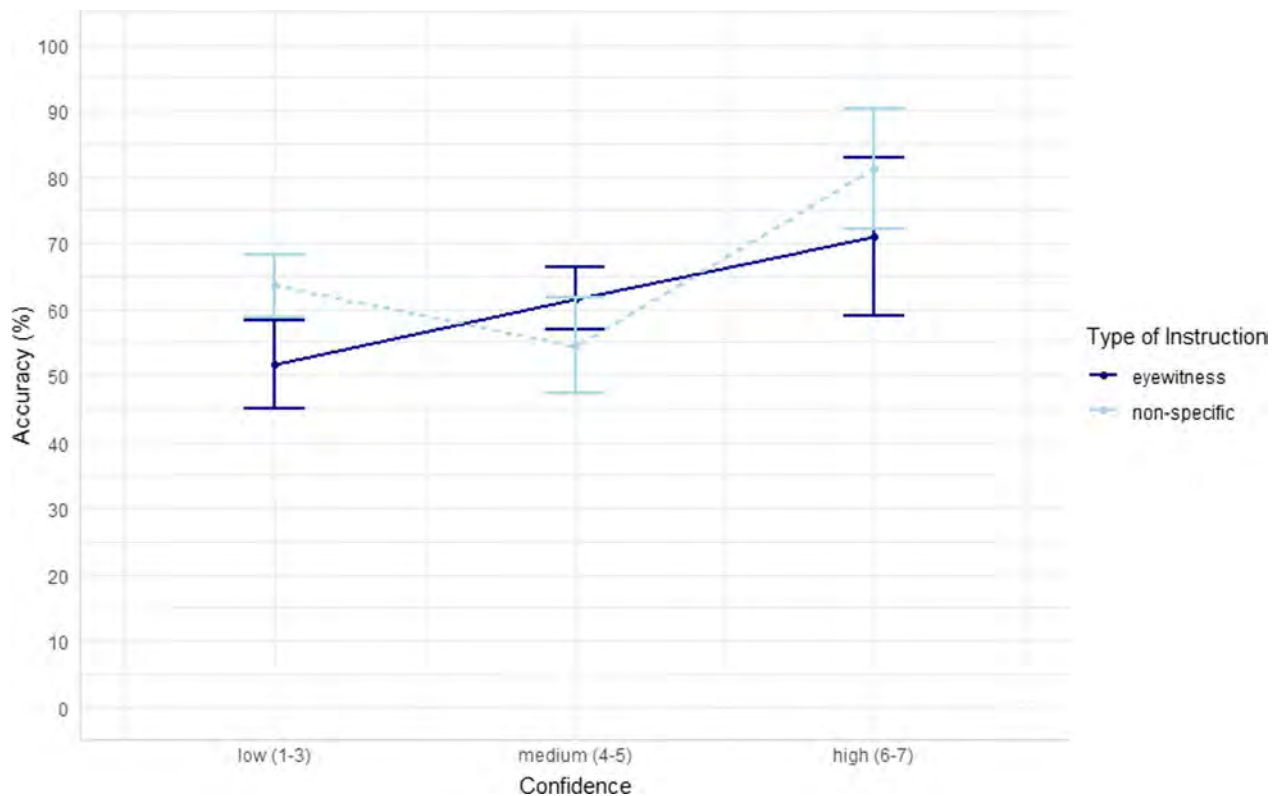
Fig. 4: 3-bin CAC
